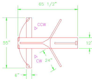
PLAN TIFFANY T80
