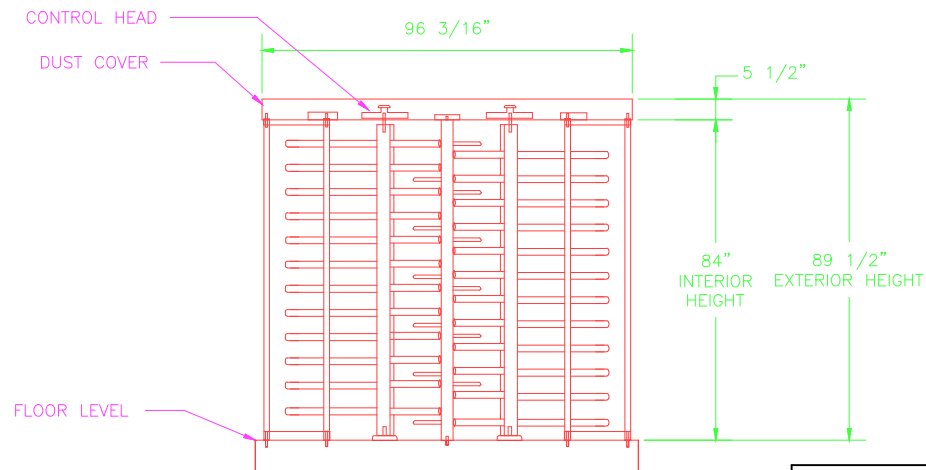
PLAN TIFFANY TWIN T80T
