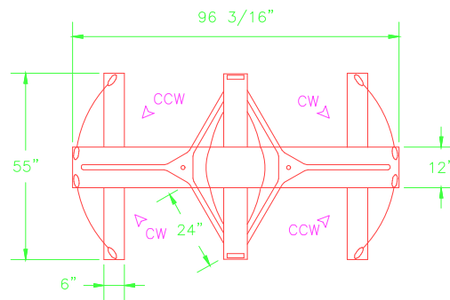
PLAN TIFFANY TWIN T80T
